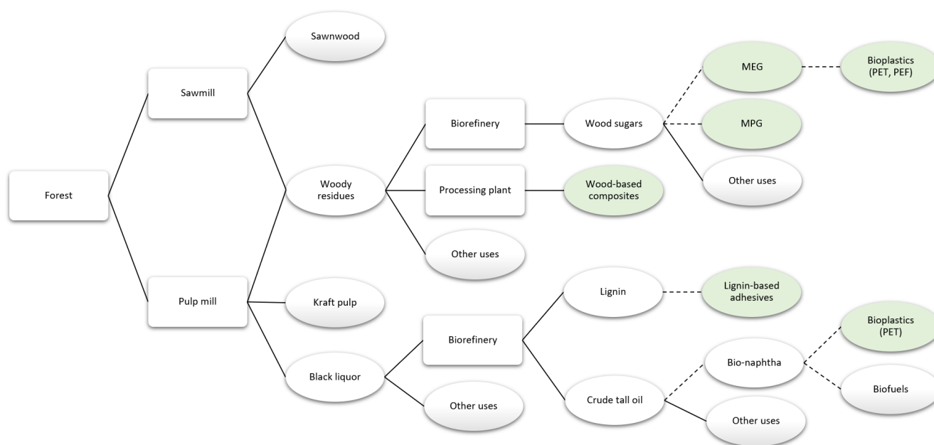
Figure 8. Simplified value chain focused on products that might use industrial sides streams as input, with the reviewed products in green. Solid lines denote existing routes and dashed lines represent potential routes. MEG is monoethylene glycol, MPG is monopropylene glycol, PET is polyethylene terephthalate, and PEF is polyethylene furanoate.
