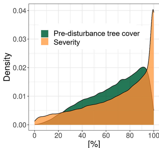
Fig. 4. Distribution of pre-disturbance tree cover and severity in the eastern Alps.
